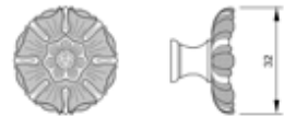
OZ1182.000.** Furniture knob - Individual sale
